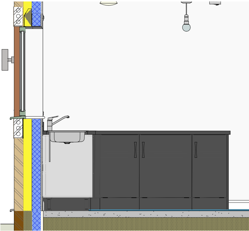
4 Kitchen - View C 1 : 25
