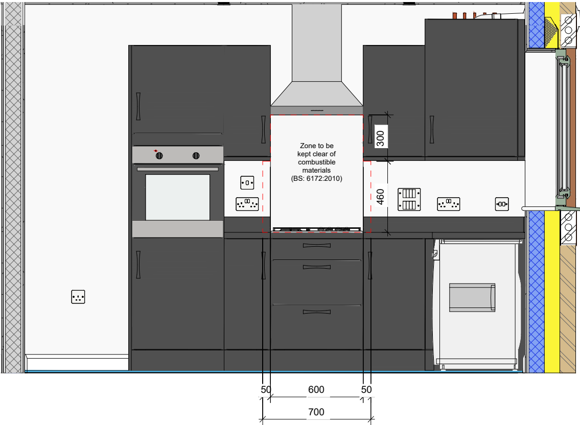
2 Kitchen - View A 1 : 25
